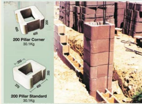
Vertical reinforcing in centre of wall and in columns as per engineers design. Stack wall to height required.
