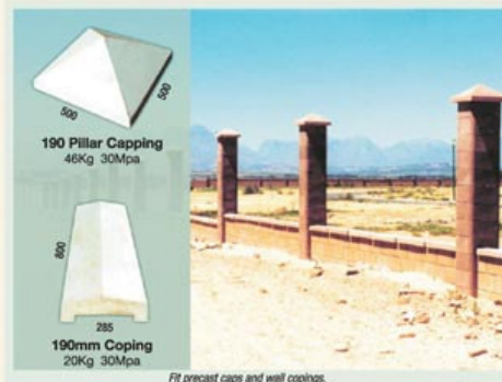
Fit precast caps and wall copings.
