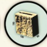
90 Half Block 4.7Kg 12.5/m.Sq 7Mpa
